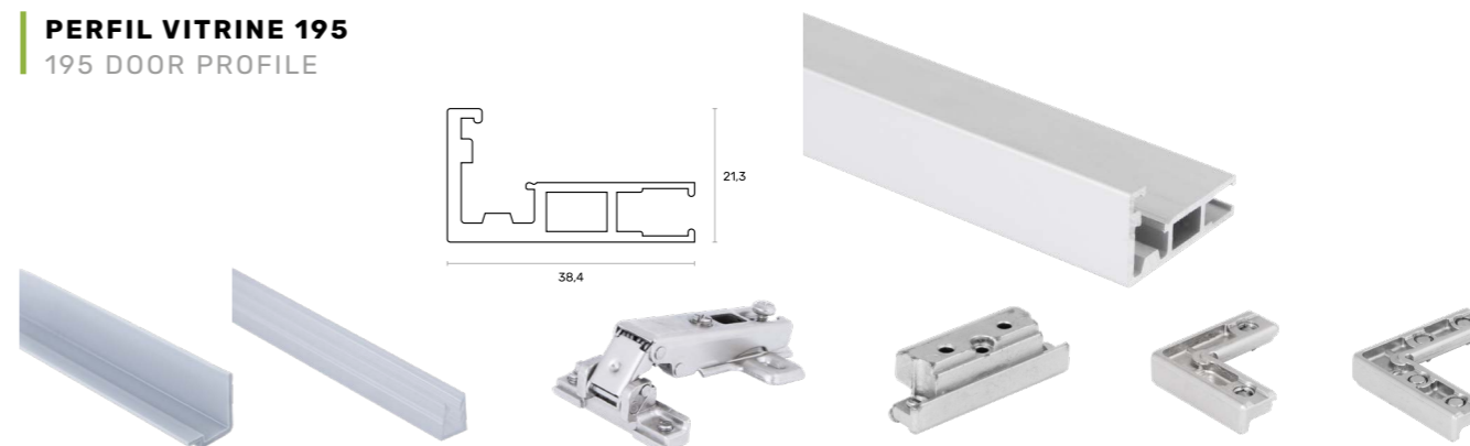
CALHAS PLÁSTICO - COBERTURA E VIDRO PROFILE FOR GLASS AND INTERNAL CARTER | DOBRADIÇA 195 195 HINGE | BASE P/COMPASSO GAS SPRING BASE | ESQUADROS MS E MSD MS AND MSD CONNECTORS
