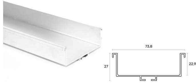
PERFIL GOLA CENTRAL 800 CENTRAL VERTICAL 800 GOLA PROFILE
